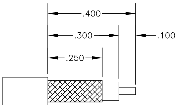
STRIPPING DIMENSIONS
