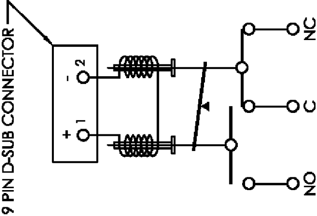
SCHEMATIC (FAILSAFE POSITION)
