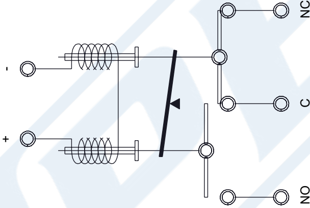
SCHEMATIC
