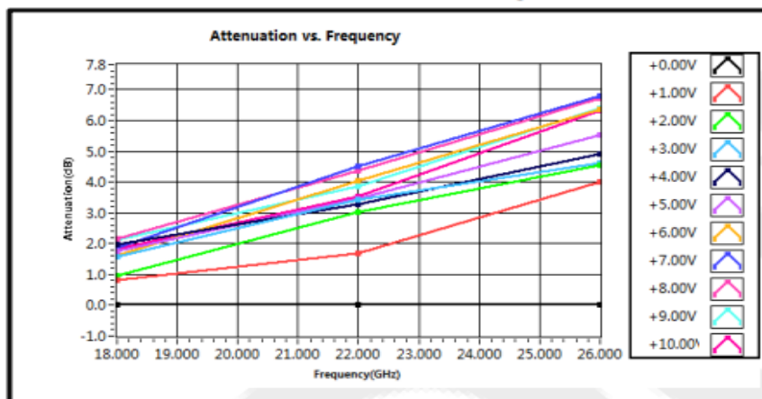
Attenuation vs. Frequency
