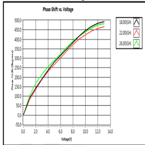
Phase Shift vs. Voltage
