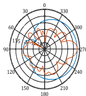
f=925MHz, Co@2-cuts
